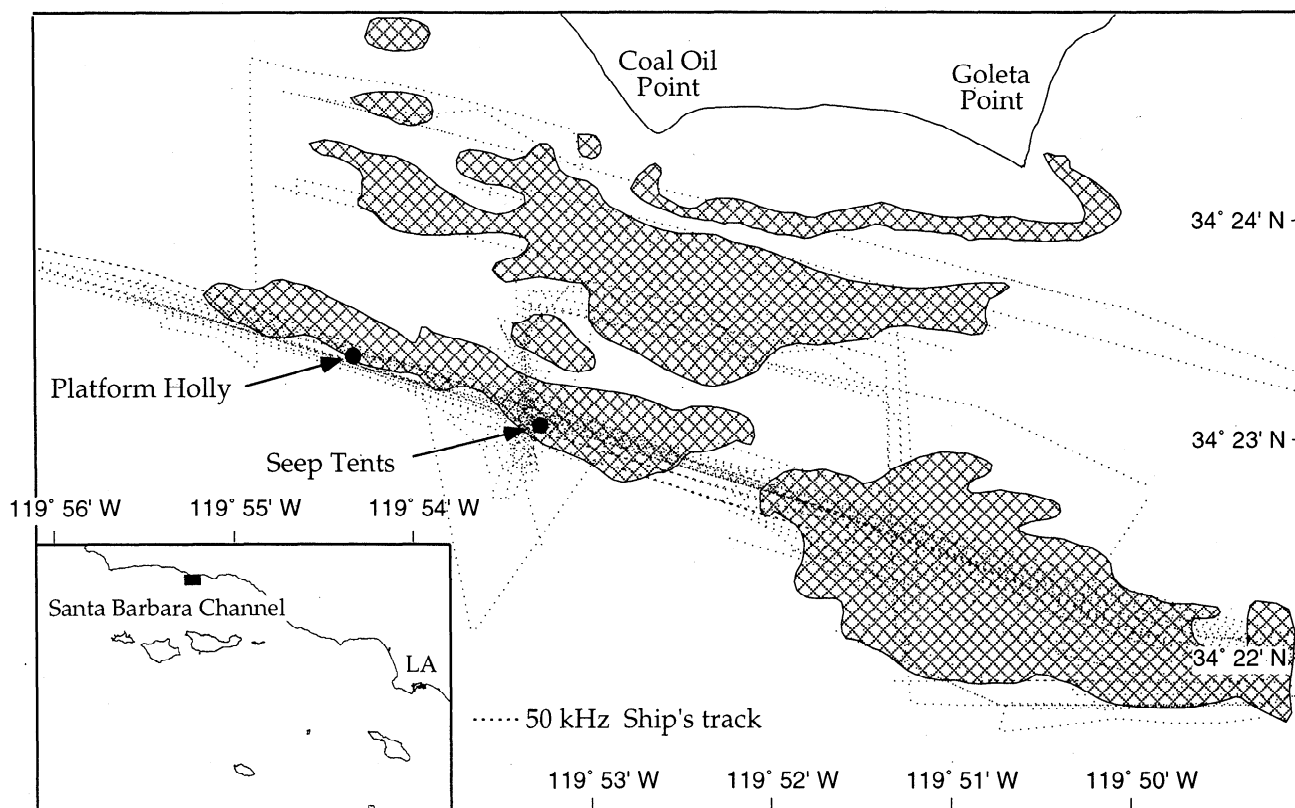
Figure 1. Locations of natural hydrocarbon seeps mapped between 1946 and 1973 offshore from Coal Oil Point near Santa Barbara [after Fischer, 1977, Fischer and Stevens, 1973]. Also shown are the locations of the seep containment tents, platform Holly, and the 50 kHz sonar track lines acquired in 1994 and 1995 that are discussed in this paper.
